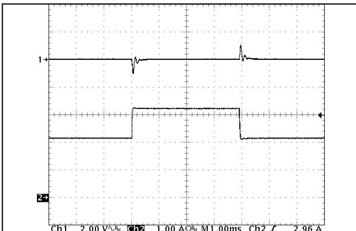
Figure 5: Output voltage response to step-change in load current (50% -75% -50% of I_{out(max)} ; dI/dt = 0.05 A/\mu s ). Load cap: 1 \mu F ceramic and 15 \mu F tantalum capacitors. Ch 1: V_{out} , Ch 2: I_{out} .
