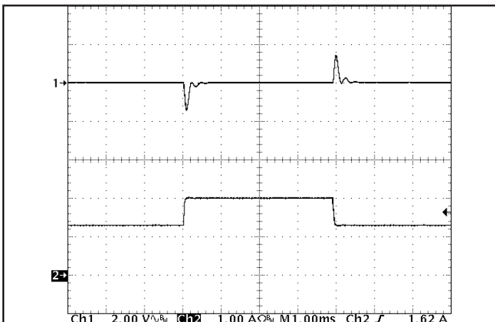
Figure 5: Output voltage response to step-change in load current (50% -75% -50% of I out (max); dI/dt = 0.02 A/μs). Load cap: 1 μF ceramic and 15 μF tantalum capacitors. Ch 1: V out , Ch 2: I out .
